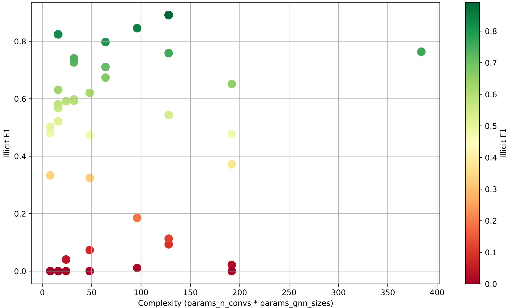
Illicit F1 vs Complexity for AMLSim 1/3
